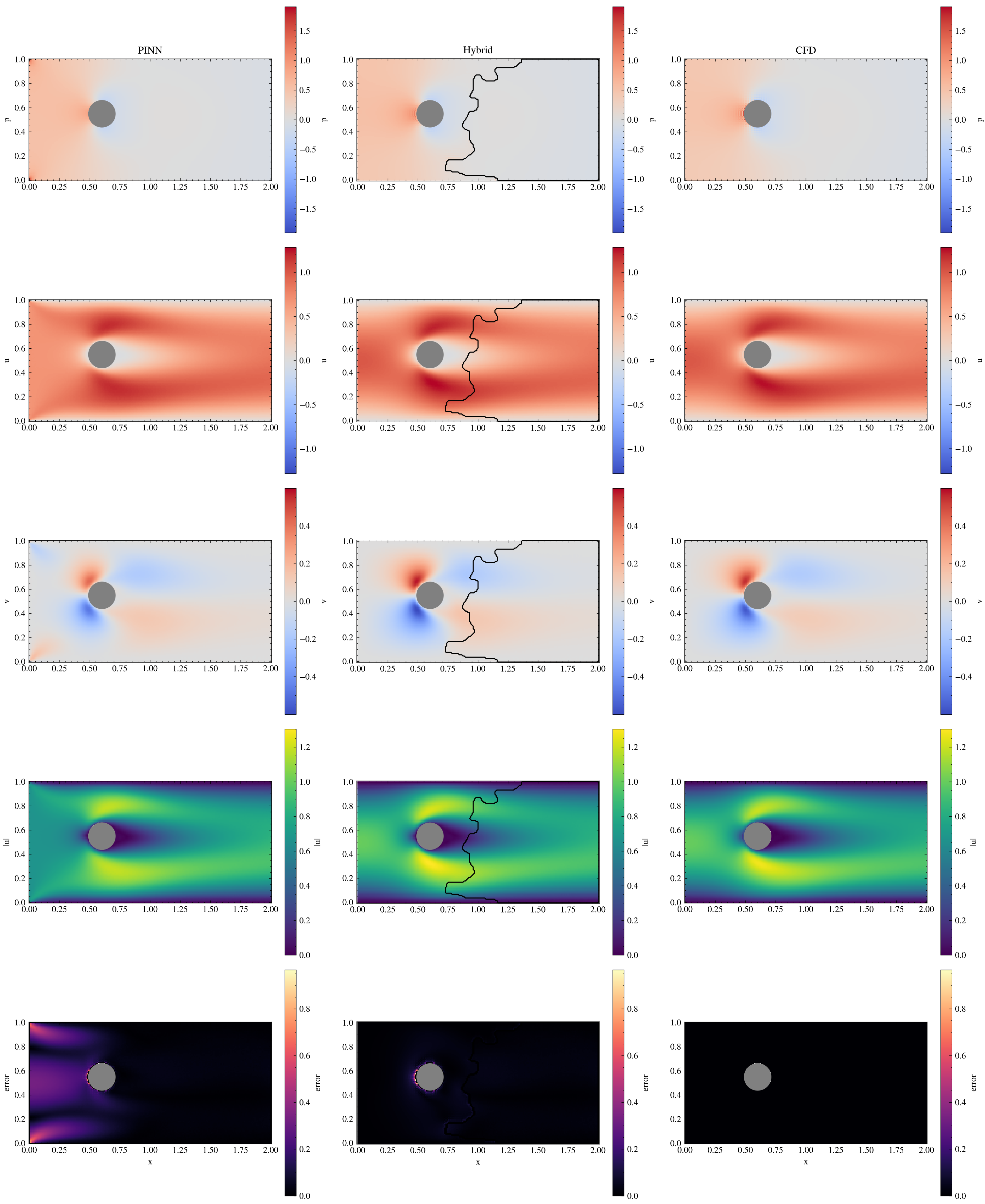
PINN vs Hybrid vs CFD (cyl=(0.6, 0.55, r=0.11), inlet u_0=1 , Re=100)
